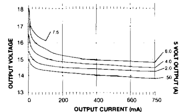
Auxiliary Load Regulation NFC40-XXT05-15
