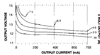
Auxiliary Load Regulation NFC40-XXT05-15
